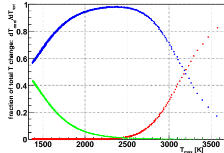
Figure 5: Relative contribution of cooling processes to the total temperature change as a function of temperature. Blue points are for radiative cooling, red for thermionic emission and green are for the heat transfer.
