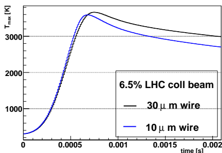
Figure 9: Distribution of wire temperature during a scan of LHC collision beam with 6.5% of the nominal intensity.
