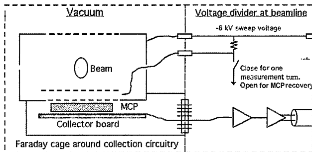
Figure 1: Schematic of detector and electronics located at the beamline.
