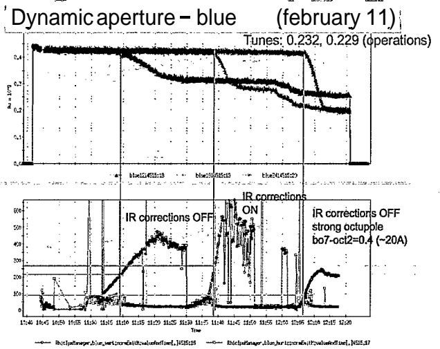
Figure 8. Dynamic aperture studies in RHIC with AU beam. Three bunches were kicked and the intensity (top) and emittance were measured. The dynamic aperture is the emittance where beam loss begins.
