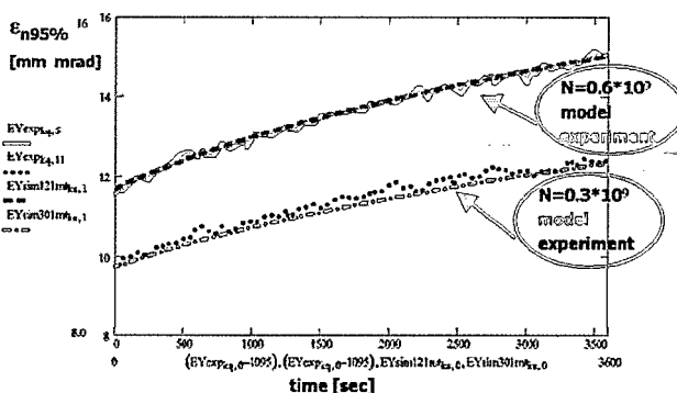
Figure 6. Plots showing emittance growth measurements compared to predicted rates from model. These data were taken over one hour on two bunches.
