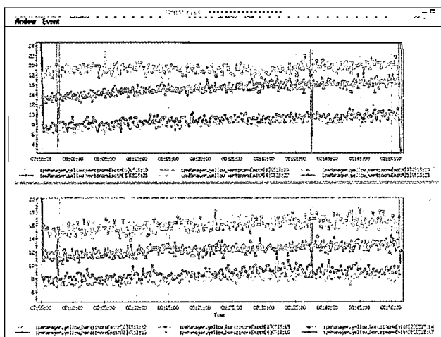
Figure 3. Simultaneous emittance measurements on six bunches of different intensities. Measurements period is one hour.
