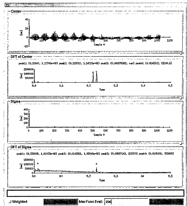
Figure 4. Power spectrum page from the application. Here the beam is being driven transversely by the ac dipole. The drive frequency is slightly different from the betatron frequency resulting in beating of the amplitude (top) and two lines in the dipole spectrum.
