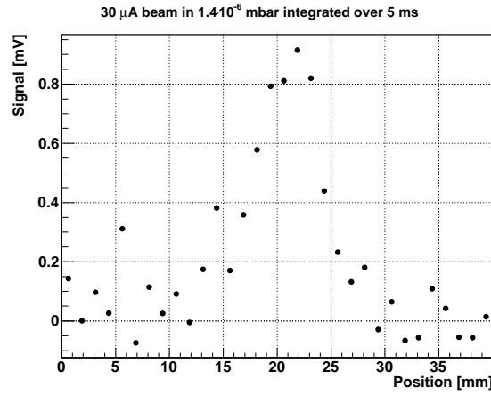
Figure 4.12: Lowest measurable IPM signal integrated over 5 ms at 30 \mu\text{A} beam current and 1.4 \cdot 10^{-6} \text{ mbar} residual gas pressure.
