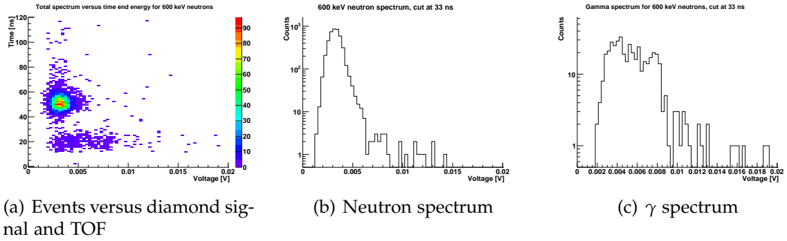
Figure A.1: 600 keV neutron energy
