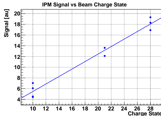
Figure 4.11: IPM signal versus the charge state of the beam particles.
