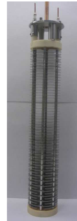
(b) Photo of the interior of the LHC IC [46].
