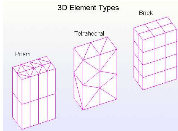
Figure 4.3: Different possible mesh types for 3D geometries.[93]
