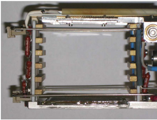
(a) Photo of the IPM prototype field box.
