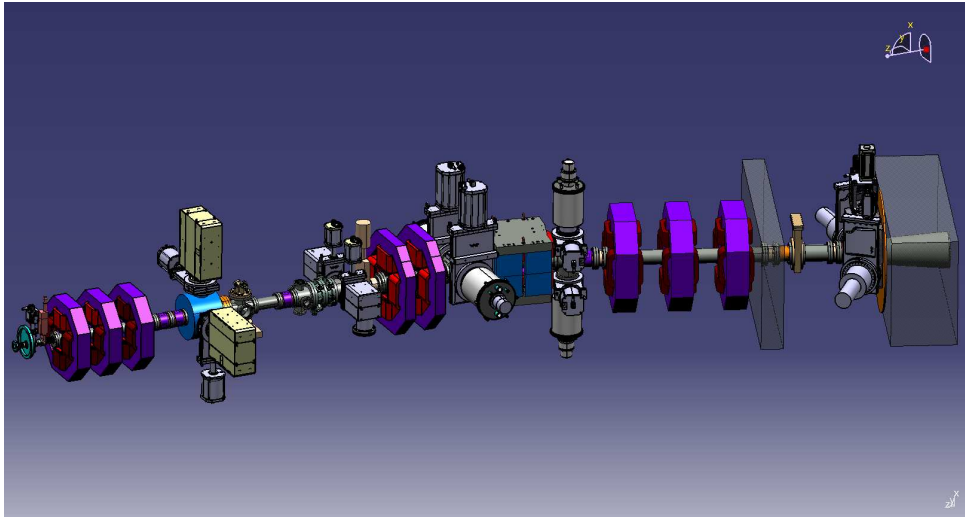
Figure 1.17: CAD Mock up of the transfer line downstream the SRF-linac, containing the quadrupole triplet, the D-plate and the quadrupole doublet to the left of the bending magnet and the rest of HEBT to the right.
