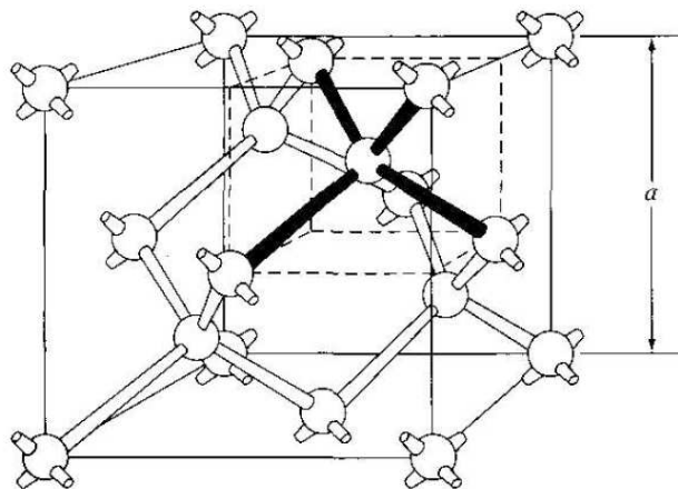
Figure 2.20: The unit cell of diamond, where a = 3.567 \text{ \AA} is the cubic lattice constant [58].
