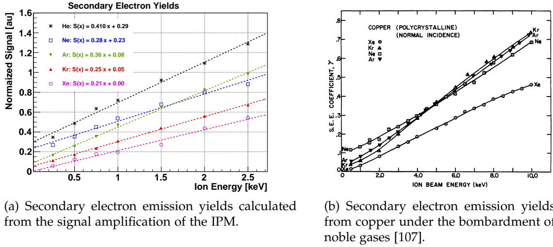
Figure 4.25: Signal amplification at stronger extraction fields and the secondary electron emission yields measured by Magnuson et al. [107].
