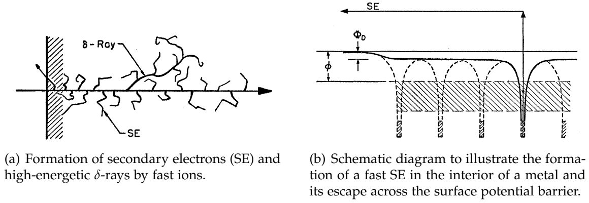
Figure 3.1: Figures illustrating the generation of secondary electrons [78].
