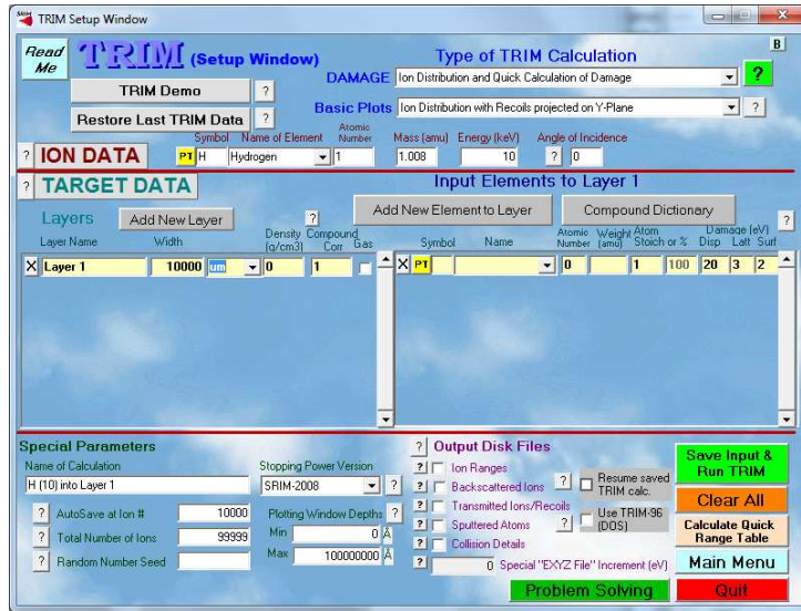
Figure 3.2: Graphical user interface of the SRIM simulation software [51].
