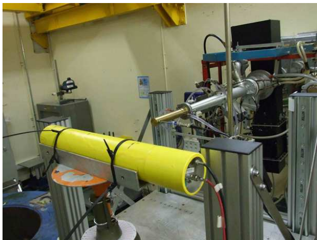
Figure 2.7: Photo of the experimental setup at the SAMES accelerator at CEA Valduc, in yellow the IC and the oscilloscope in the background the accelerator with the D/T-target.
