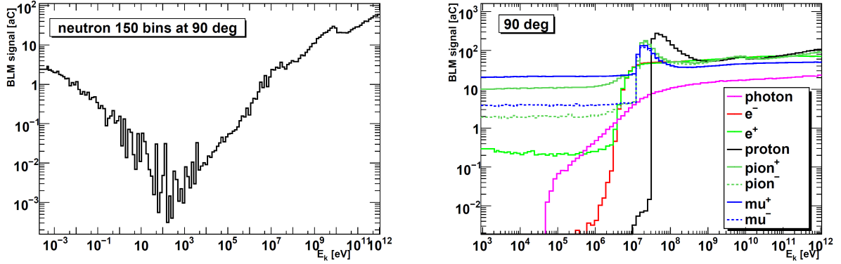
Figure 2.5: Response function of the LHC IC for various primary particles and energies [50].
