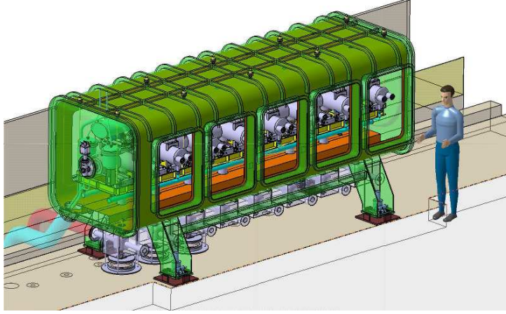
Figure 1.10: Sketch of the IFMIF first cryomodule that constitutes the SRF-linac of the prototype accelerator. inside [28].
