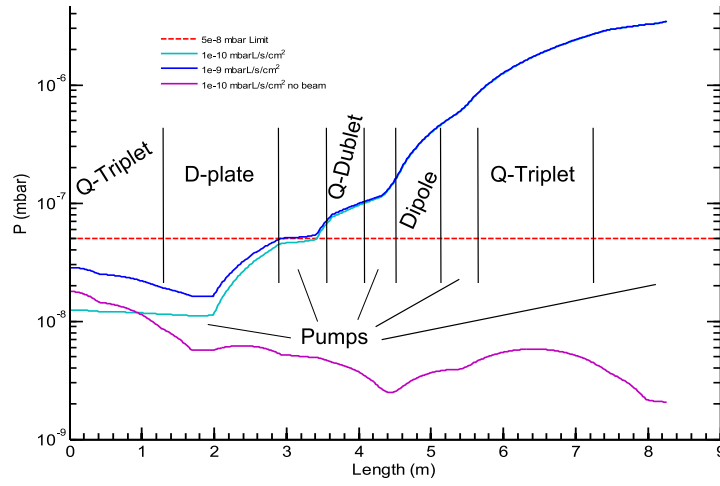
Figure 4.32: Expected vacuum pressure downstream the SRF linac indicating also the quadrupole dublet / triplets, the D-plate, and the bending dipole [111].
