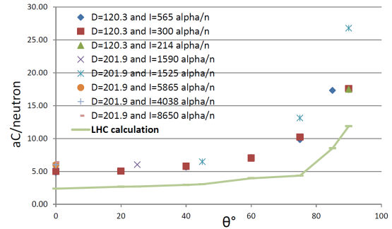
(b) Response Function for 14.1 MeV neutrons.
