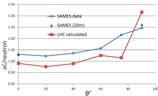
(a) Response Function for 2.45 MeV neutrons.
