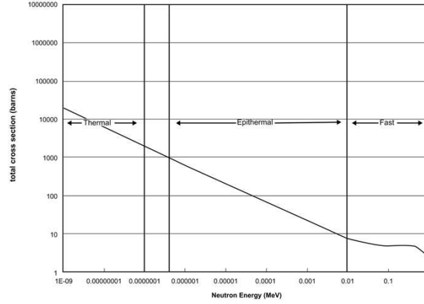
Figure 2.13: Neutron capture cross section of ^{10}\text{B} [53].
