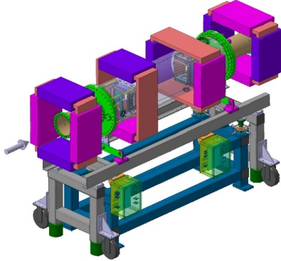
(a) Design drawing of the GSI IPM [82].
