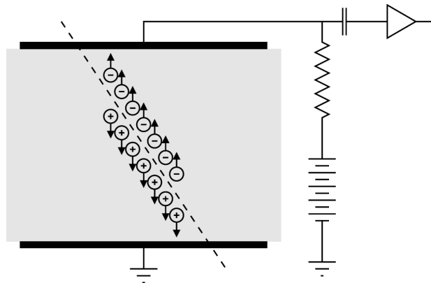
Figure 2.21: An ionizing particle passes through a diamond detector. It generates electron-hole pairs that are extracted by an electric field applied over electrodes on top and on bottom [59].
