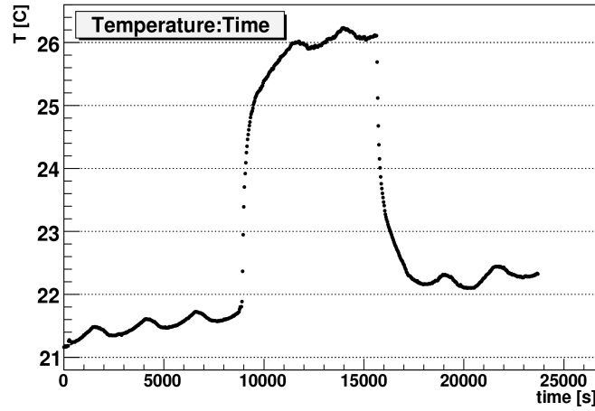
Figure 4: Example of a heating curve for the sensor 10A64A8E000800FB.
