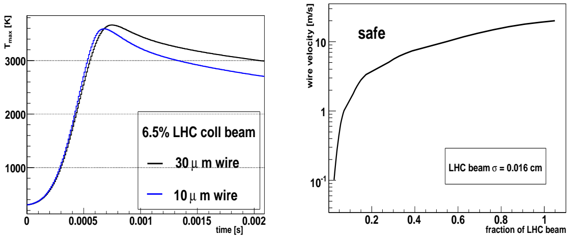
Figure 12: Left plot: evolution of maximum wire temperature during the scan. Blue curve shows temperature evolution for 10 \mu\text{m} wire. Right plot: the region of safe operation of the Wire Scanner for LHC collision beam.
