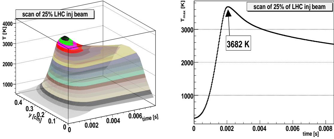
Figure 11: Left plot: distribution of wire temperature during a scan of LHC injection beam with 25% of the nominal intensity. Right plot: the same but for the maximum temperature bin.
