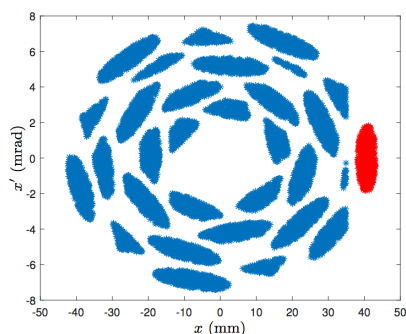
Figure 2: Multi-turn injection simulations from [7].
