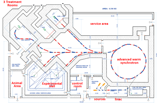
Figure 2: SEEIIST Layout.
