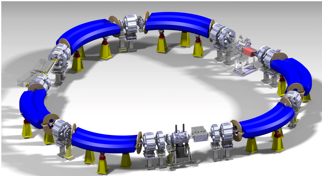
Figure 1: Layout of the HeLICS synchrotron.
