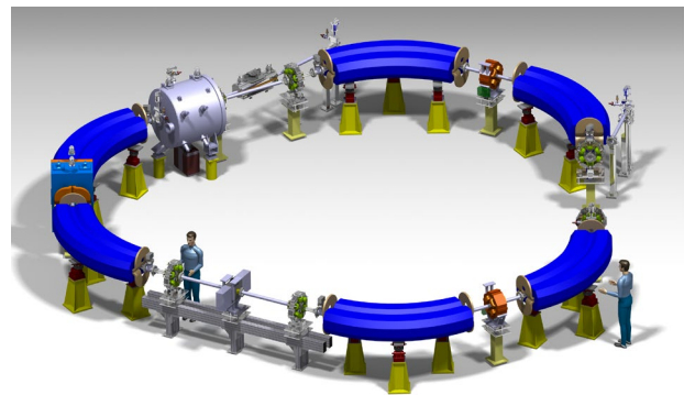
Figure 4: View of the 33 m circumference synchrotron.
