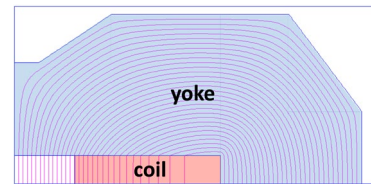
Figure 3. Dipole magnet cross section (one quarter).
