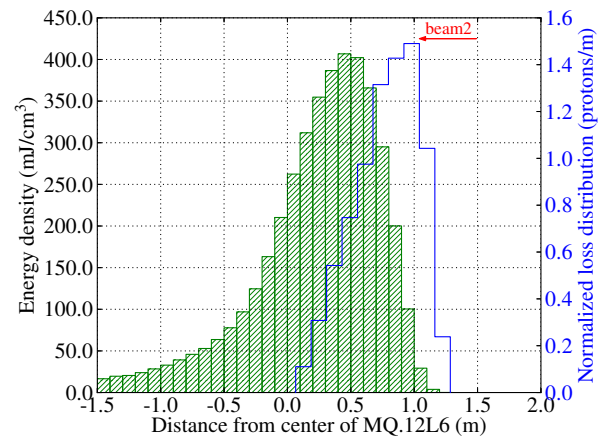
Figure 4: Peak longitudinal profile of energy density in MQ coils during the millisecond quench test. Dose values are normalized to 8.2 \times 10^8 protons. Loss distribution as predicted by MAD-X studies [11].
