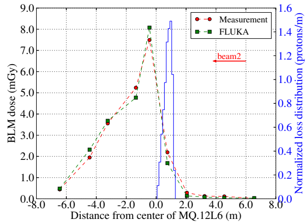
Figure 3: Comparison of simulated and measured BLM dose during the millisecond quench test. Dose values are normalized to 8.2 \times 10^8 protons. The histogram indicates proton loss distribution on the MQ beam screen as predicted by MAD-X studies [11].
