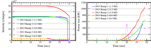
Figure 3: Beam intensity and peak power loss for the quench tests at 3.5 TeV and 4 TeV in 2011 and 2013.
