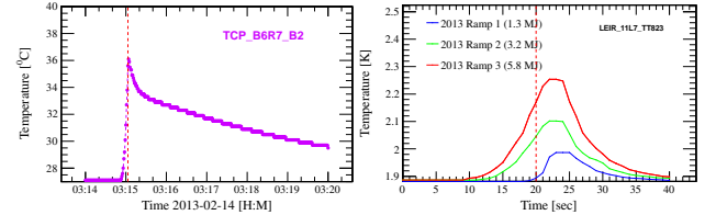
Figure 5: Temperatures in the right-downstream jaw of the skew B2 TCP for the last ramp and the empty cryostats.
