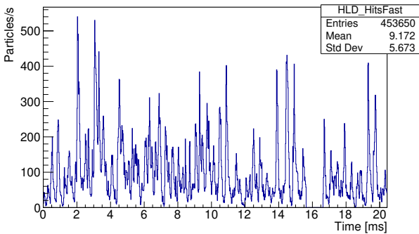
Figure 5: Micro-spill time structure of the particle rates.
