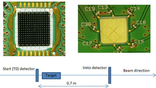
Figure 1: Arrangement of the scCVD diamond sensors in the HADES experiment. In the upper left a close-up picture of the T0 sensor is shown. The metallization which is arranged in sixteen stripes is clearly visible. The upper right corner shows a close-up picture of the scCVD diamond based veto detector with a boxed shaped metallization.
