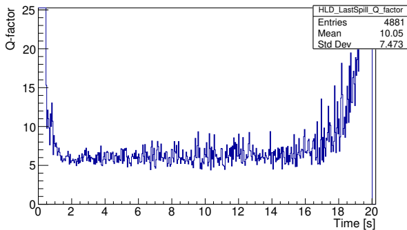
Figure 6: Quality factor of the Ar beam, which is defined by the ratio between the peak and average event rates.
