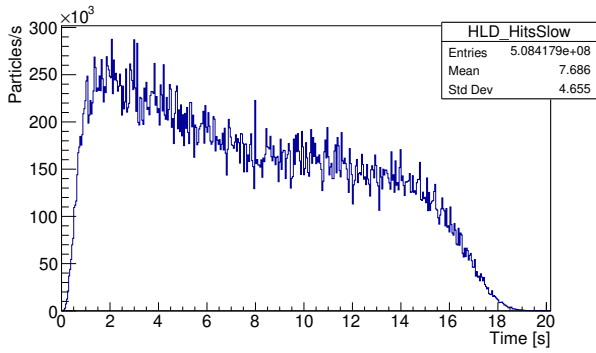
Figure 4: Macro-spill time structure measured by the sc-CVD diamond sensor in front of the HADES target. The ion particles are extracted from the SIS18 accelerator via a so called "slow extraction" in about 19 s. The maximal average rate should not be above 10^6 particles/s.
