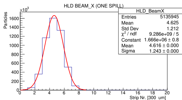
Figure 3: Beam profile measurement of an ^{107}\text{Ag}^{45+} ion beam with an energy of 1.58 A GeV using a scCVD with a metallization segmented into sixteen stripes. Each bin corresponds to a width of 300\ \mu\text{m} .
