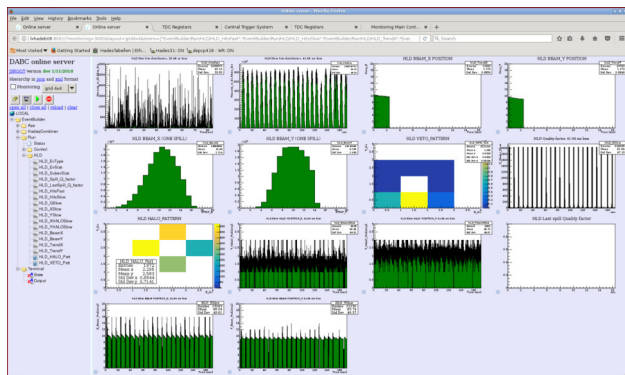
Figure 2: Important beam properties (i.e. x - and y - profile macro- and micro-spill structure) can be displayed live in any web browser.
