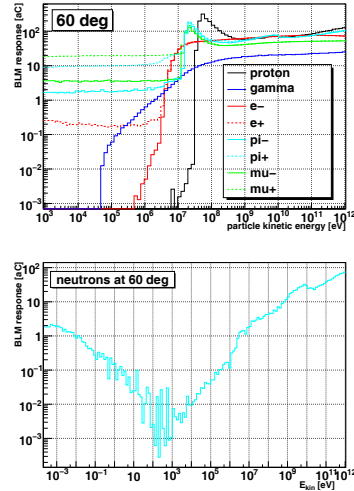
Figure 6: Response functions for 60^\circ impact angle. Top: All considered particle types except neutrons. Bottom: Neutrons only.
