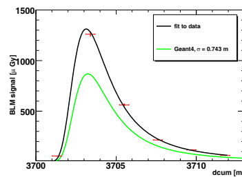
Figure 10: Second Quench causing loss signal with Landau fit curve and Geant 4 simulated ionisation chamber detector signals.
