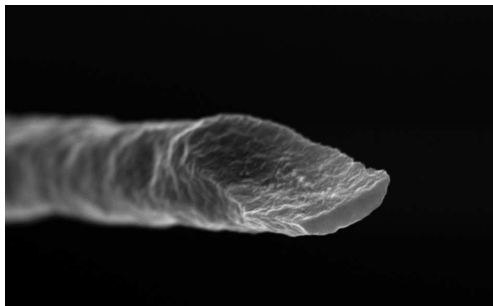
Figure 11: The carbon fiber after the experiment with ions.
