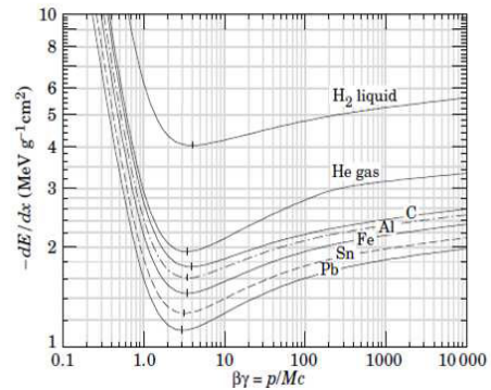
Figure 1: dE/dx for heavy particle crossing matter [1].
