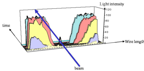
Figure 3: Pattern of RF heating of a 8 μm carbon fiber in the LEP wire scanner [2].
