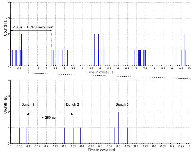
Figure 5: Ionisation electron counts as a function of time for a 10 \mu s (top) and 1 \mu s (bottom) window. The signal for each PS revolution is clearly visible in the top plot, while the signal for each individual bunch is visible in the bottom plot.
