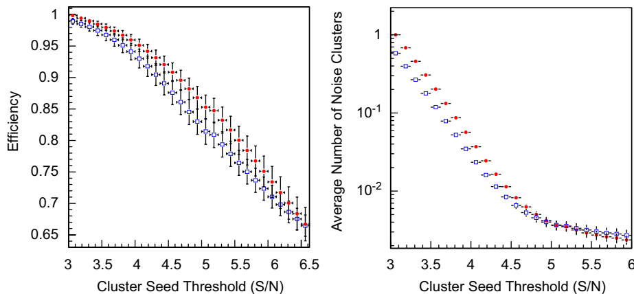
Fig. 22. On the left, detection efficiencies of the p- ( \bullet ) and n-sides ( \square ) as a function of the cluster seed threshold. On the right, the average number of noise clusters for the p- ( \bullet ) and n-sides ( \square ) as a function of the cluster seed threshold.
