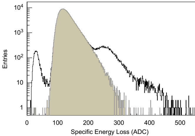
Fig. 25. The p-side specific energy loss distribution of the ladder in position 2 in the A/Z = 2 nuclei beam obtained with the light ion selection criteria (unshaded) and the distribution of the selected helium nuclei (shaded).
