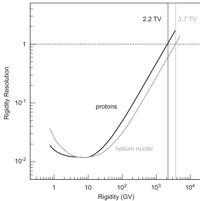
Fig. 37. The expected AMS-02 proton and helium nuclei rigidity resolutions; the values of the maximum detectable rigidity (100% measurement error) are indicated.
