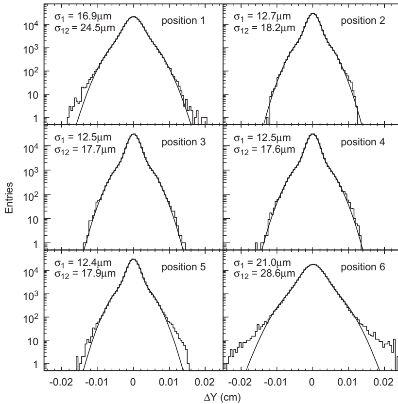
Fig. 15. The p-side residual distributions (five point fit) at the six ladder positions for the proton data of the October 2003 test beam. The residual distributions are described with a sum of two Gaussians; the narrower Gaussian width ( \sigma_1 ) and the area-weighted average width of the two Gaussians are indicated ( \sigma_{12} ).
