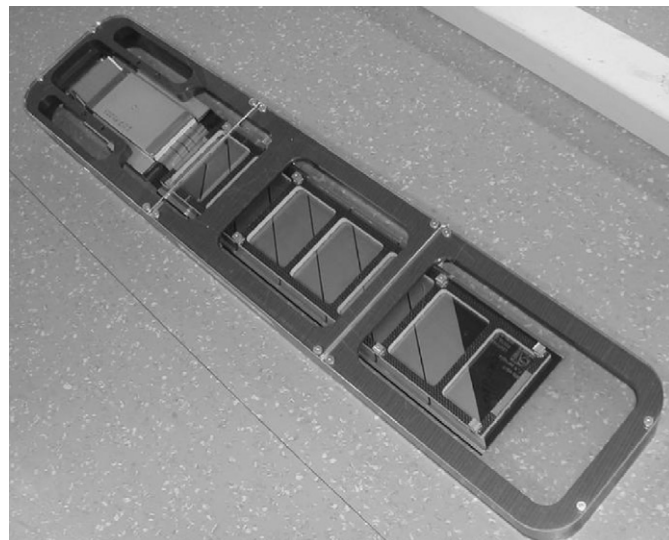
Fig. 3. View of the n-side of a seven-sensor-long AMS-02 ladder in its storage/transportation box.
