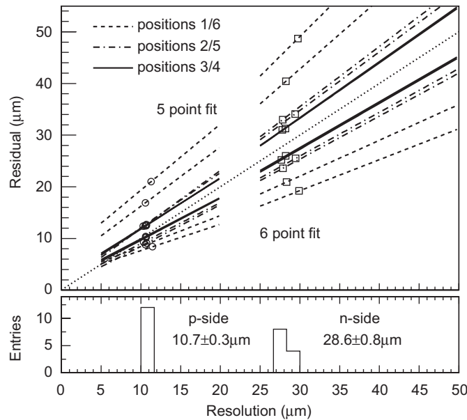
Fig. 17. The relation between proton residual widths and position resolution at the six ladder positions in the October 2003 test beam. The lines with slopes larger (smaller) than unity correspond to the five (six) point track fits. The individual ladder resolutions, corresponding to the experimental narrow Gaussian residual widths, are given by the abscissa values of the data points for the p- ( \circ ) and n-sides ( \square ). The distributions of the latter, the average values and standard deviations are shown at the bottom.
