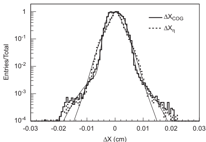
Fig. 32. The n-side helium nuclei residual distributions, and corresponding three-Gaussian fits, at the ladder in position 5 obtained with the two-strip center-of-gravity (COG) and f(\eta) .
