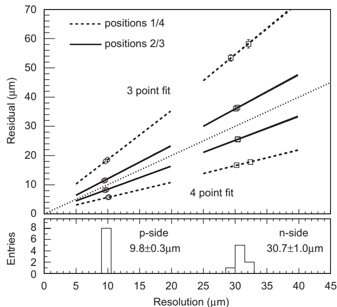
Fig. 13. The relation between residual widths and position resolution at the four ladder positions in the June 2003 test beam. The lines with slopes larger (smaller) than unity correspond to the three (four) point track fits. The individual ladder resolutions, corresponding to the experimental narrow Gaussian residual widths, are given by the abscissa values of the data points for the p- ( \circ ) and n-sides ( \square ). The distributions of the latter, the average values and standard deviations are shown at the bottom.
