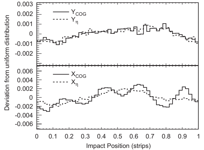
Fig. 20. The reconstructed impact position on the p- (top) and n-sides (bottom) of the ladder at position 2 obtained with the center-of-gravity (COG) and f(\eta) (dashed line). The bin contents represent the fractional difference with respect to a uniform distribution.
