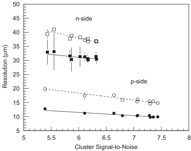
Fig. 34. Optimal (closed symbols) and effective (open symbols) position resolutions as a function of the cluster signal-to-noise from the June 2003 proton data.
