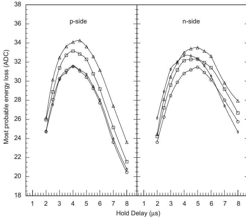
Fig. 9. Most probable specific energy loss as a function of the VA hold delay for the four ladders present in the June 2003 test beam.
