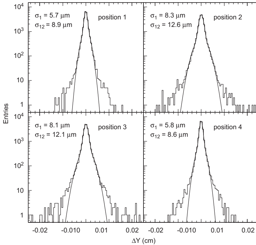
Fig. 11. The p-side residual distributions (four point fit) at the four ladder positions for the 4\mu\text{s} hold delay data of the June 2003 test beam. The residual distributions are described with a sum of two Gaussians; the narrower Gaussian width ( \sigma_1 ) and the area-weighted average width of the two Gaussians are indicated ( \sigma_{12} ).
