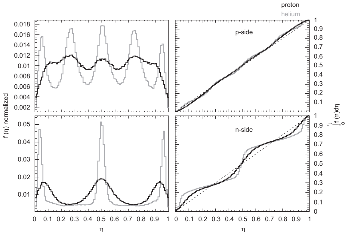
Fig. 19. On the left, the proton and helium normalized \eta distributions of the p- (top) and n-sides (bottom); on the right, the integral values of f(\eta) which describe the correlation between the track position in the readout gap and relative signal amplitudes of the two strips. The dashed lines of unit slope indicate the appropriate correlation for the position obtained with the center-of-gravity of the strip signals.
