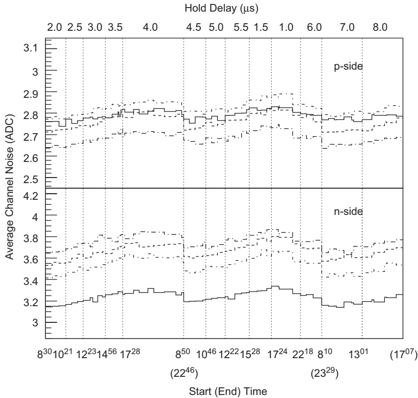
Fig. 6. The evolution in time (hour and minutes indicated) of the average strip noise of the four ladders present in the June 2003 test beam. The noise levels display a daily variation due to the temperature changes in the experimental hall. The corresponding VA hold delays of the different data periods are indicated at the top.
