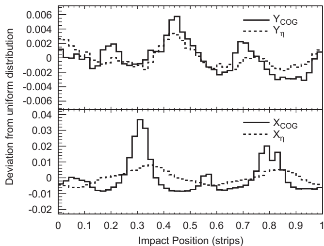
Fig. 31. The reconstructed impact position of the helium nuclei tracks on the p- (top) and n-sides (bottom) of the ladder at position 5 obtained with the center-of-gravity (COG) and f(\eta) (dashed line). The bin contents represent the fractional difference with respect to a uniform distribution.
