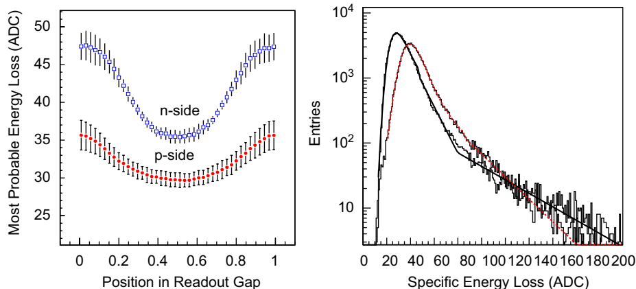
Fig. 23. On the left, the most probable specific energy loss as a function of the proton position in the readout gap for the p- (●) and n-sides (□). On the right, the proton specific energy loss on the n-side of the ladder in position 3 in the October 2003 test beam, and the Gaussian-convoluted Landau fit (including a high energy exponential tail) which is used to describe the energy loss distribution in the two regions of the readout gap: IP < 0.2 and IP > 0.8 (dashed line) and 0.4 ≤ IP ≤ 0.6 (solid line).
