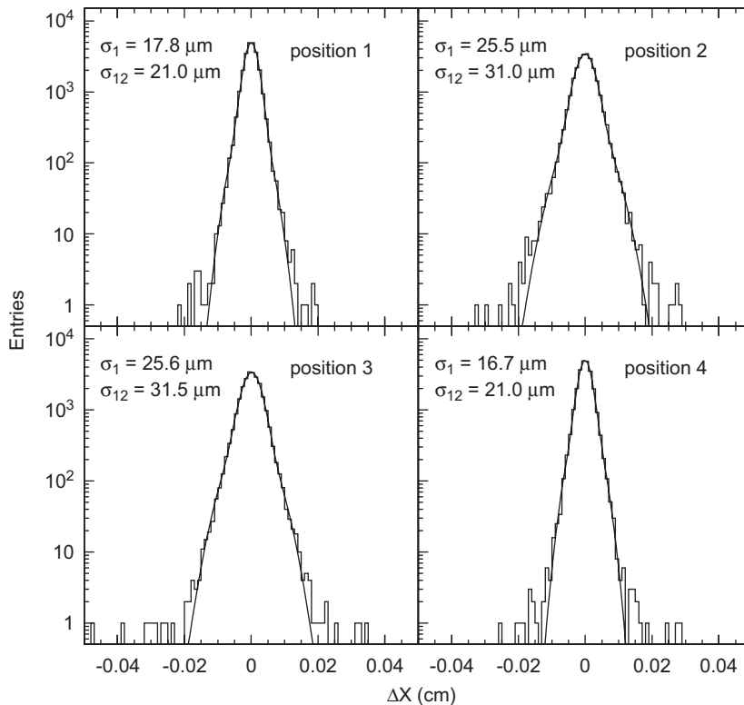
Fig. 12. The n-side residual distributions (four point fit) at the four ladder positions for the 4\mu\text{s} hold delay data of the June 2003 test beam. The residual distributions are described with a sum of two Gaussians; the narrower Gaussian width ( \sigma_1 ) and the area-weighted average width of the two Gaussians are indicated ( \sigma_{12} ).
