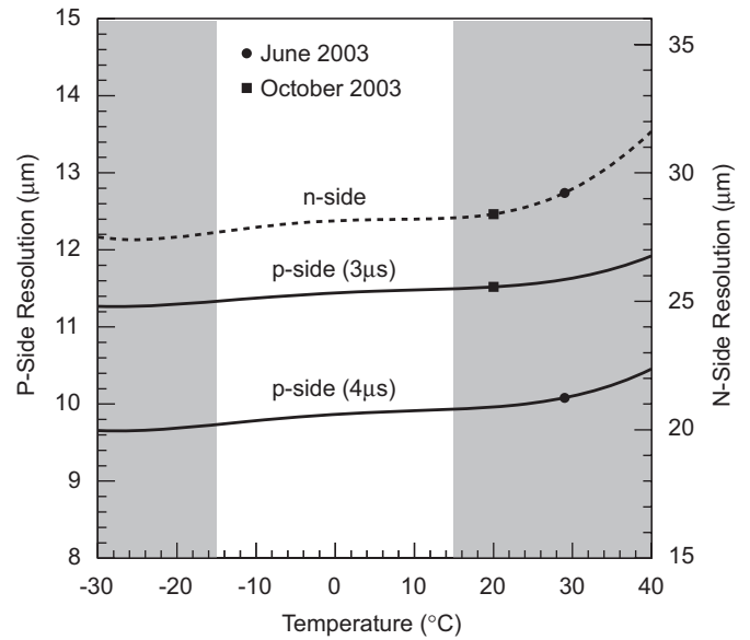
Fig. 35. Position resolution for singly charged relativistic particles (normal incidence) as a function of the temperature; the p-side (solid) and n-side (dashed) resolutions are indicated on the left and right, respectively. Results for delay hold times of 3 and 4 µs are shown for the p-side. The operating conditions and corresponding resolutions are indicated for the June and October 2003 test beams. The unshaded region corresponds to the expected operating temperature range of the tracker on the ISS.
