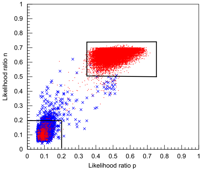
Fig. 28. The distribution of the likelihood ratios, \mathcal{L}_{2,3}^n and \mathcal{L}_{2,3}^p , computed for the helium ( \times ) and lithium ( \cdot ) nuclei samples. The boxes denote the charge selections applied to determine efficiencies and contamination levels for the two nuclei.
