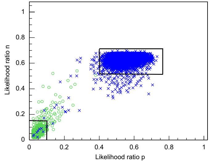
Fig. 27. The distribution of the likelihood ratios, \mathcal{L}_{1,2}^p and \mathcal{L}_{1,2}^n , computed for the proton ( \circ ) and helium nuclei ( \times ) samples. The boxes denote the charge selections applied to determine efficiencies and contamination levels for the singly and doubly charged particles.
