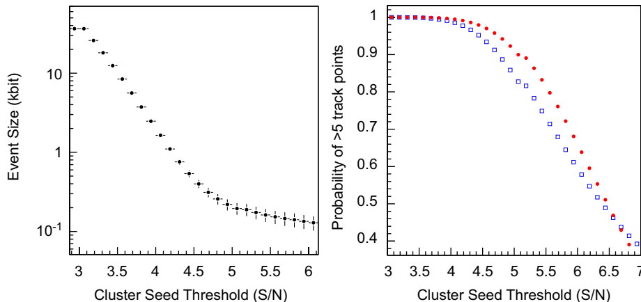
Fig. 38. On the left, the contribution of the tracker noise clusters to the AMS-02 event size as a function of the threshold of the cluster seed strip. On the right, the probability of >5 measurements on the p- ( \bullet ) and n-sides ( \square ) of the ladders along the particle path as a function of the threshold of the cluster seed strip. Threshold levels are expressed in terms of the single channel noise ( \sigma_{\text{ped}} ); the results are based on the ladder performance in the October 2003 test beam (Fig. 22).
