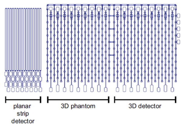
Fig. 1. Mask for the metallisation of the diamond sample [4]. It is divided into three parts. On the right a strip structure to connect all conductive channels (“3D detector”), which is repeated in the middle but without conductive channels underneath (“3D phantom”) and on the left a planar strip detector.
