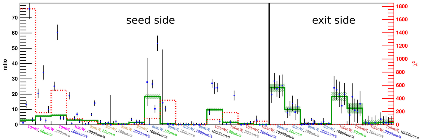
Fig. 3. Ratio of the value of the diamond peak to the value of the g -peak. Results for individual channels are marked by a blue cross, the weighted mean for each setting is indicated by the green line. The red dotted line shows the \chi^2 value for each setting. (For interpretation of the references to color in this figure caption, the reader is referred to the web version of this paper.)
